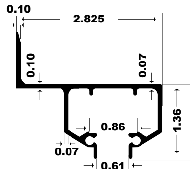
367 - 1" WALL HEADER
