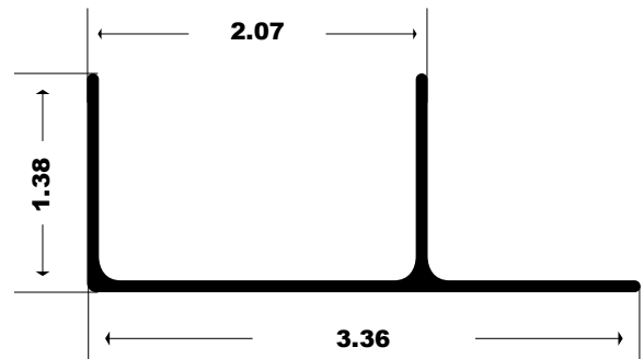
357 - ADJUSTABLE BOTTOM
