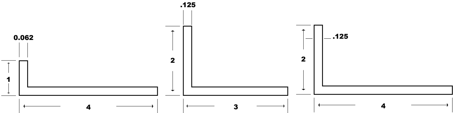
108 - 1"x 4" x .062 ANGLE
