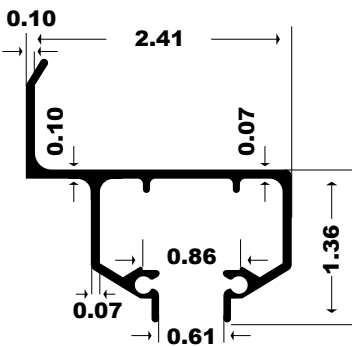
366 - 5/8" WALL HEADER
