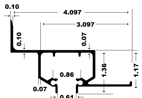
353 - 1" WALL HEADER RAINGUARD
