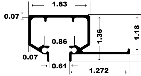
354 - CEILING HEADER RAINGUARD
