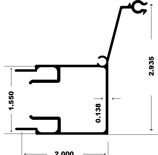
335 - HI TECH MALE CM
