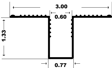
358 - RECESSED TRACK
