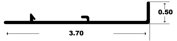
365 - DIRECT MOUNT 2"
