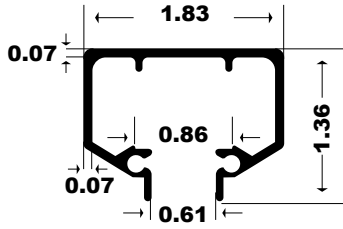
368 - CEILING HEADER
