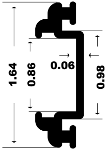
362 - COMMERCIAL INSERT
